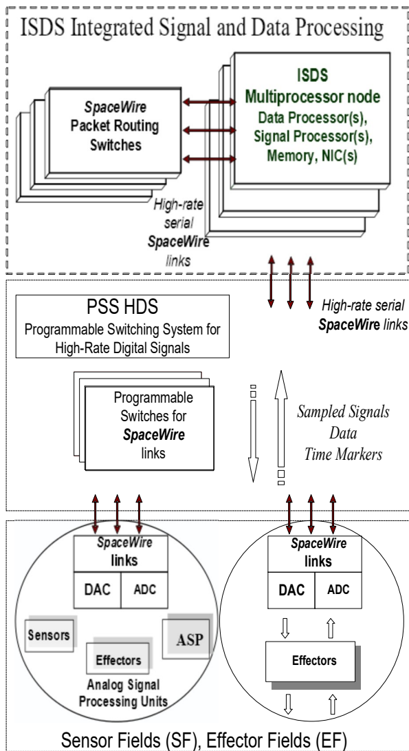
Fig. 1. Distributed Integrated Modular Spacecraft Avionics Architecture
