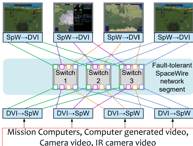
Fig. 5 Fault tolerant fly-by-wire systems; 2 failures tolerant cockpit interconnection
