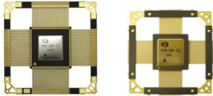
Fig.2 A micropocessor and peripheral controller with embedded SpaceWire/ GigaSpaceWire links
