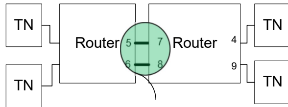
Fig.4 Adaptive routing by port number
